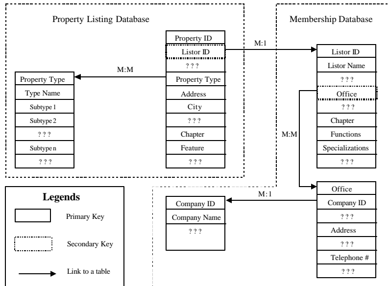
Figure 4: A Simplified Data Model for COMMREX
