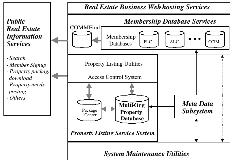
Figure 3: COMMREX Logical Structure
