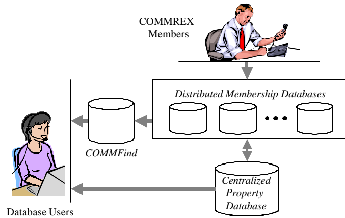
Figure 2. COMMREX Data allocation
